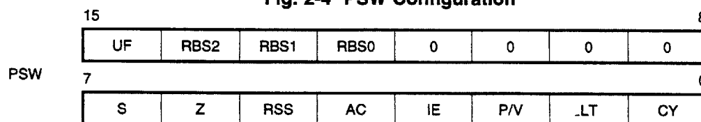
Fig. 2-4 PSW Configuration
