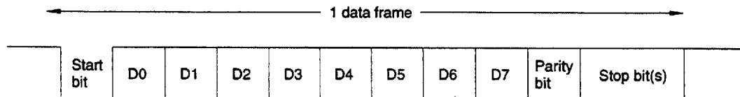
Fig. 4-18 Data Transmission Format for the Asynchronous Serial Interface
