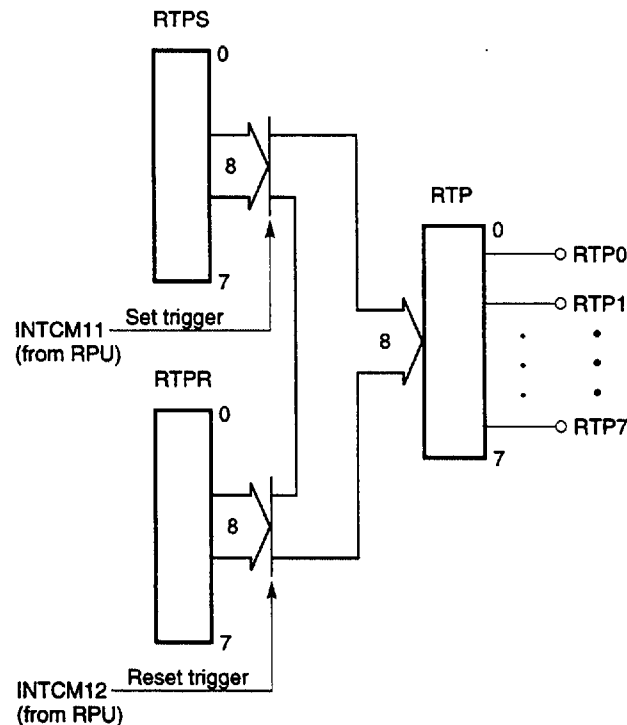
Fig. 4-11 Outline of the Real-time Output Port
