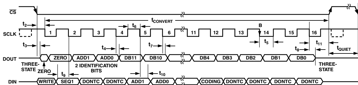
Figure 16. Serial Interface Timing Diagram
