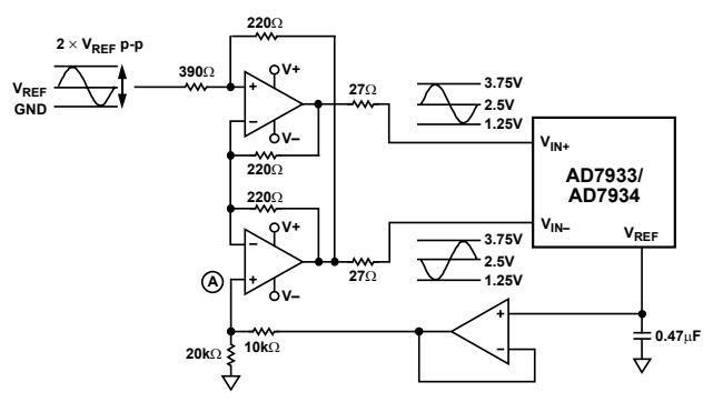
Figure 30. Dual Op Amp Circuit to Convert a Single-Ended Unipolar Signal into a Differential Signal
