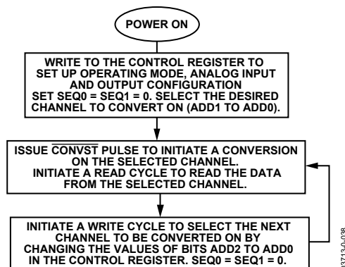
Figure 33. Normal Multichannel Operation Flow Chart
