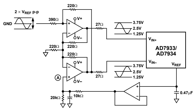
Figure 31. Dual Op Amp Circuit to Convert a Single-Ended Bipolar Signal into a Differential Signal
