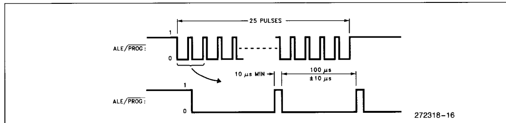
Figure 9. PROG Waveforms
