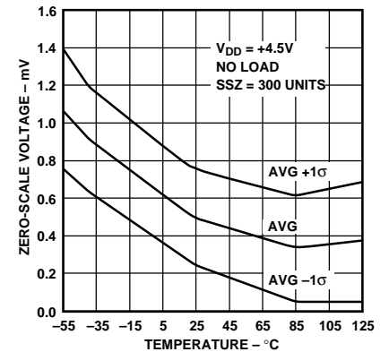
Figure 17. Zero-Scale Voltage vs. Temperature
