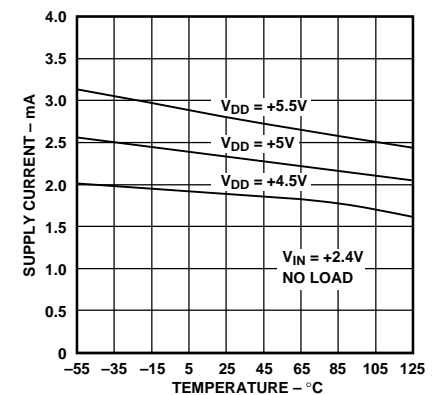
Figure 20. Supply Current vs. Temperature
