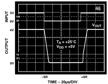
Figure 14. Large Signal Settling Time
