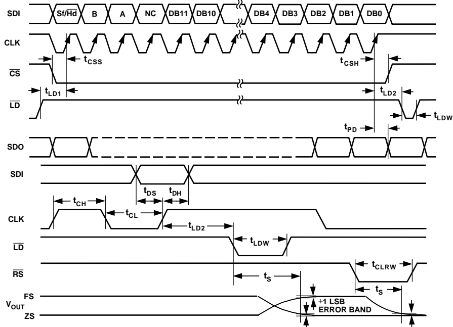
Figure 2. Timing Diagram
