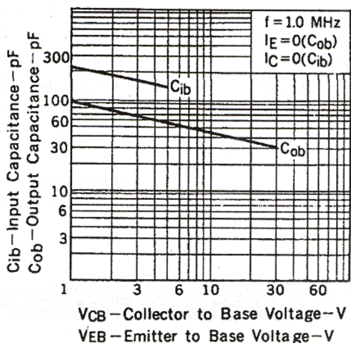
INPUT AND OUTPUT CAPACITANCE vs. REVERSE VOLTAGE
