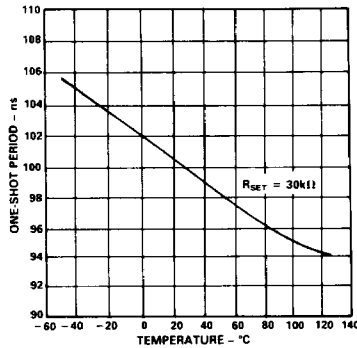
Figure 8. One-Shot Period vs. Temperature
