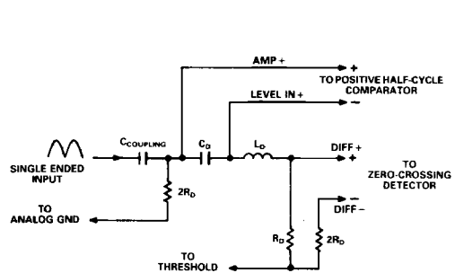
Figure 11b. Single-Ended Configuration of Passive Delay-Line Differentiator
