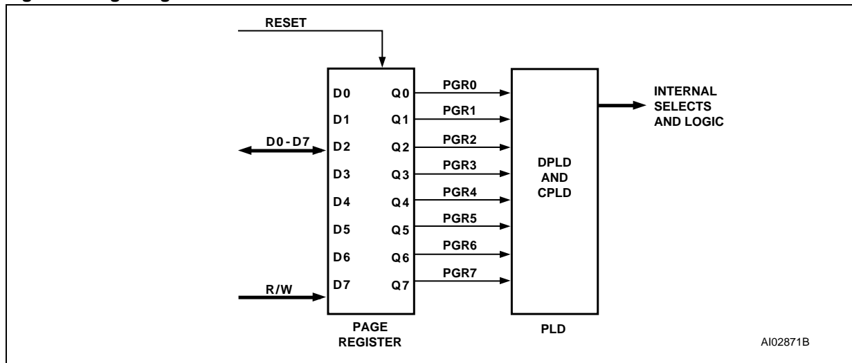
Figure 9. Page Register
