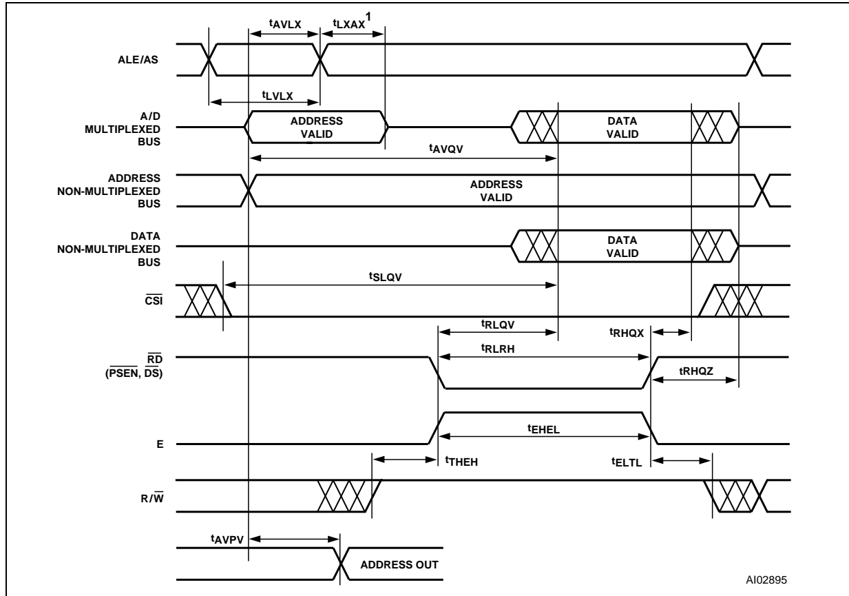
Figure 41. Read Timing
