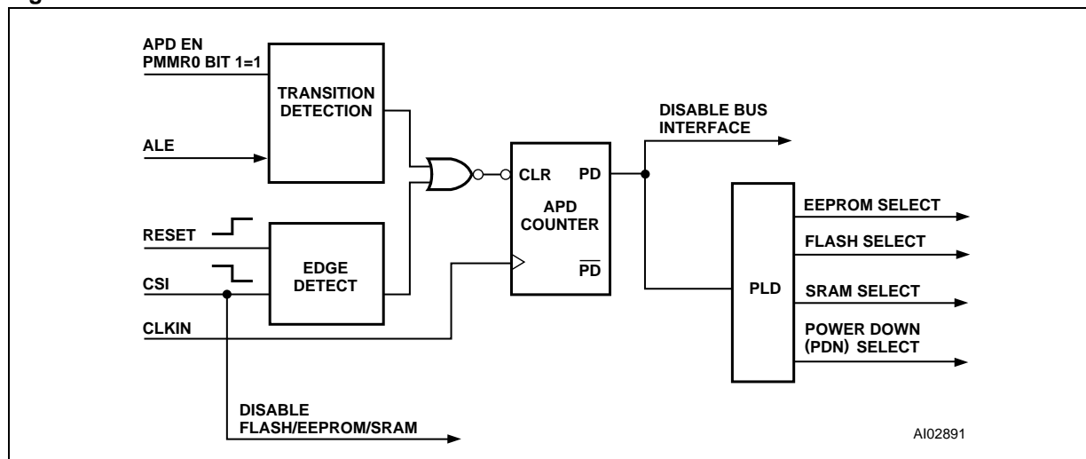
Figure 29. APD Unit
