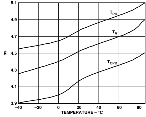
TPC 14. T_{PD} , T_V , T_{CPD} vs. Temperature
