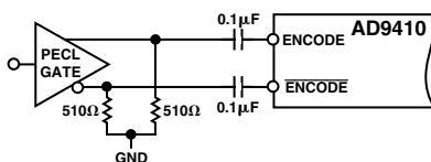
Figure 11. Driving the Encode Inputs Differentially
