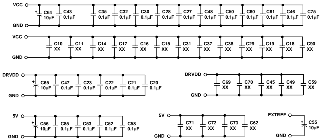
Figure 49. LVDS Mode Evaluation Board Schematic (Continued)
