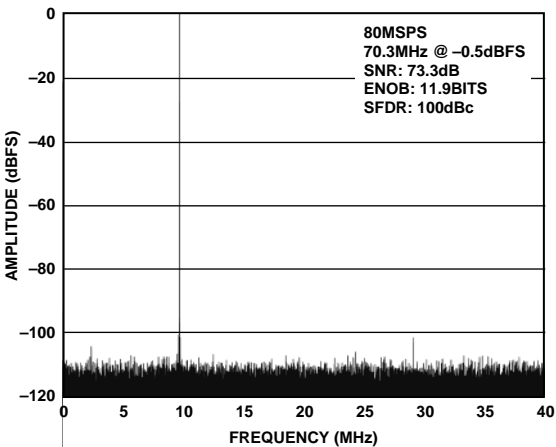
Figure 14. 64K Point Single-Tone FFT/80 MSPS/70 MHz
