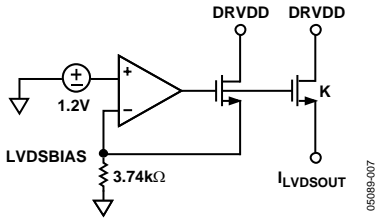
Figure 7. Equivalent LVDS BIAS Circuit
