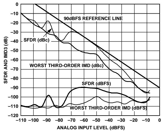
Figure 28. Two-Tone SFDR vs. Analog Input Level, A_{IN} = 69.3 \text{ MHz}/70.3 \text{ MHz}
