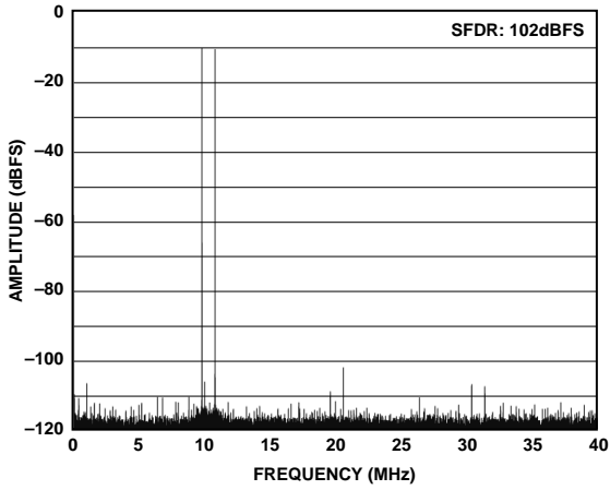
Figure 24. 32K Point Two-Tone FFT 80 MSPS/9.8 MHz/10.8 MHz
