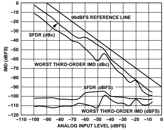
Figure 27. Two-Tone SFDR vs. Analog Input Level, A_{IN} = 9.8 \text{ MHz}/10.8 \text{ MHz}
