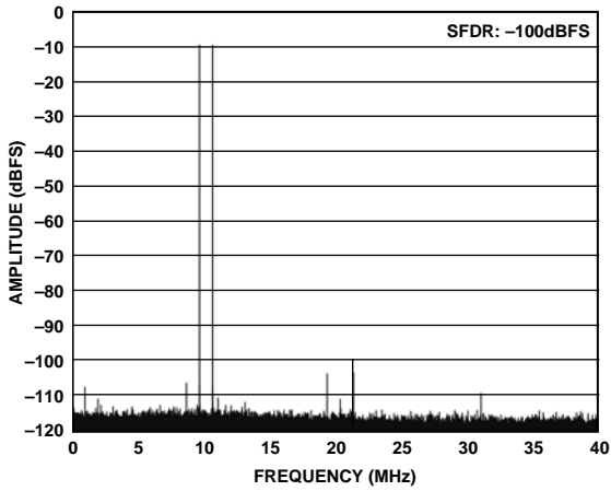
Figure 25. 32K Point Two-Tone FFT 80 MSPS/69.3 MHz/70.3 MHz
