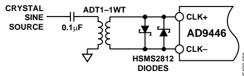
Figure 59. Crystal Clock Oscillator, Differential Encode
