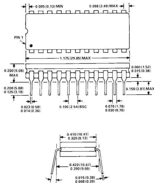
22-Pin Ceramic DIP
