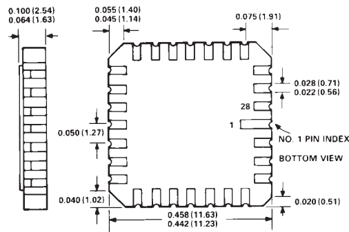
28-Pin LCC
