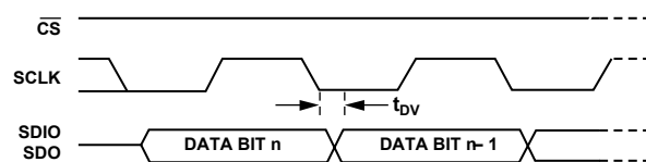
Figure 12. Timing Diagram for Register READ to AD9725
