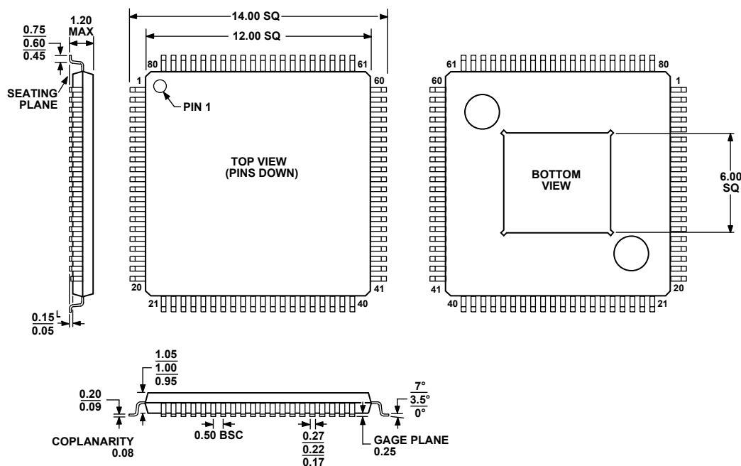
Figure 13. 80-Lead Thin Plastic Quad Flat Package, Exposed Pad [TQFP/ED] (SV-80)
