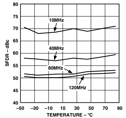
TPC 15. SFDR vs. Temperature, f_{DAC} = 300 MSPS @ 0 dBFS
