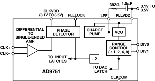
Figure 6. Clock Circuitry with PLL Active
