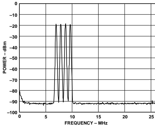
Figure 49. Spectral Plot of AD9772 Reconstructing Four GSM Modulated Carriers @ f_{\text{DATA}} = 52 \text{ MSPS} , \text{PLL}_{\text{VDD}} = 0
