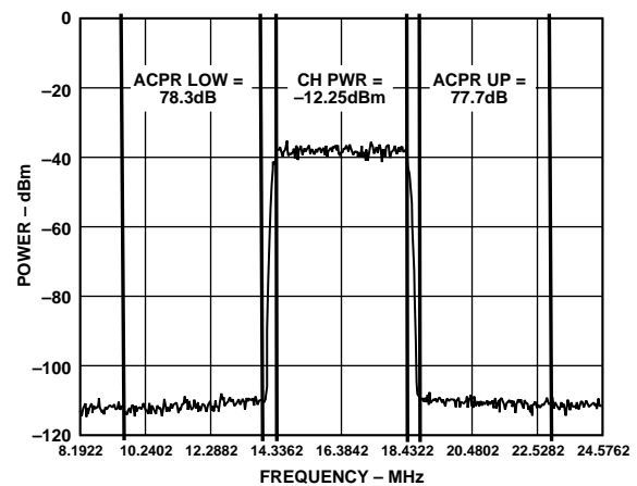
Figure 50. AD9772 Achieves 78 dB ACPR Performance Reconstructing a "WCDMA-Like" Test Vector with f_{\text{DATA}} = 65.536 \text{ MSPS} and \text{PLL}_{\text{VDD}} = 0
