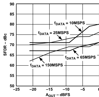
Figure 17. "In-Band" Dual-Tone SFDR vs. A_{OUT} @ f_{OUT} = f_{DATA}/3
