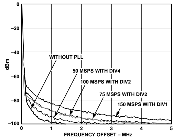
Figure 27. Phase Noise of PLL Clock Multiplier @ Exactly f_{\text{OUT}} = f_{\text{DATA}}/4 at Different f_{\text{DATA}} Settings with Optimum DIV0/DIV1 Settings Using R & S FSEA30 Spectrum Analyzer
