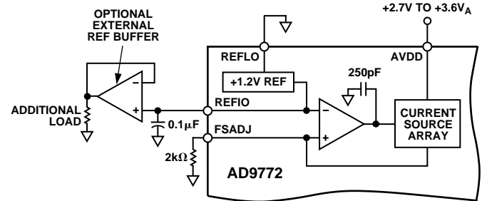
Figure 32. Internal Reference Configuration
