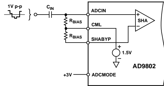
Figure 23. AC-Coupled Input
