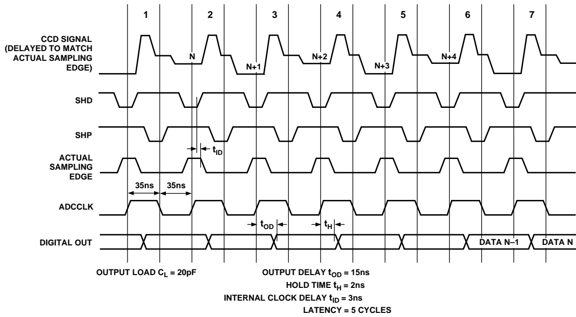
Figure 12. Timing Diagram
