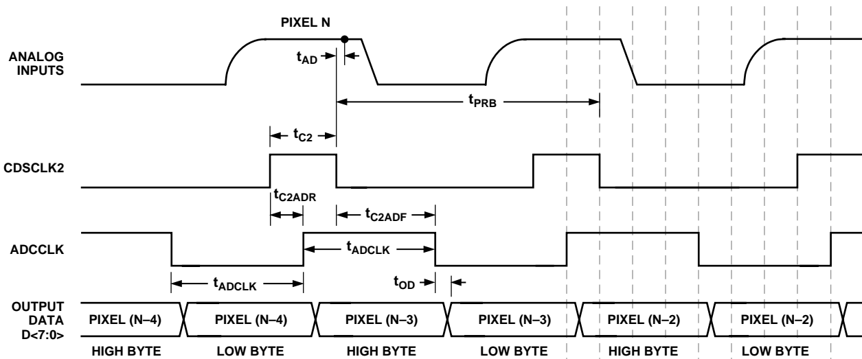
Figure 4. 1-Channel SHA Mode Timing
