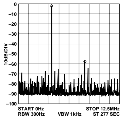
Figure 15. f_{MCLK} = 25 \text{ MHz} , f_{OUT} = 4.1 \text{ MHz} , Frequency Word = 29FBE76D
