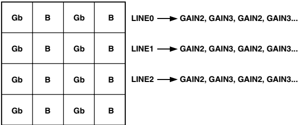
Figure 18b. CCD Color Filter Example: Interlaced
