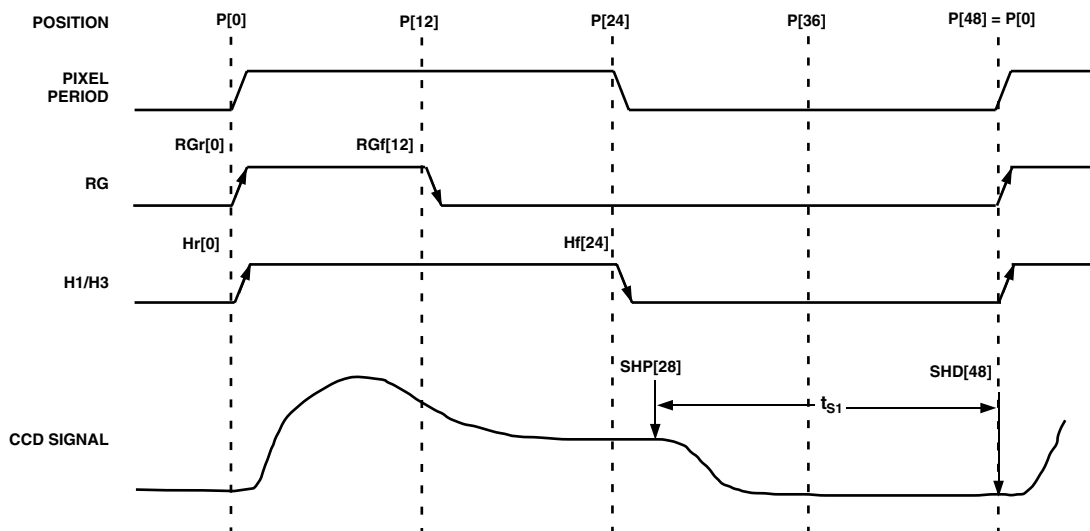
Figure 6. High-Speed Clock Default and Programmable Locations
