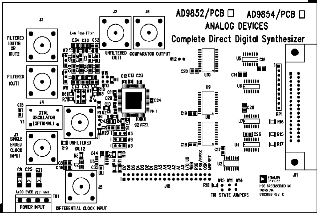
Figure 63. Assembly Drawing
