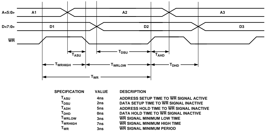
Figure 50. Parallel Port Write Timing Diagram
