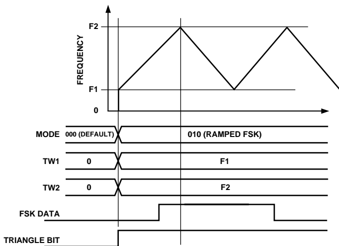
Figure 42. Automatic Linear Ramping Using the Triangle Bit Additional flexibility in the ramped FSK mode is provided in the ability to respond to changes in the 48-bit delta frequency word and/or the 20-bit ramp-rate counter on-the-fly during the ramping from F1 to F2 or vice versa. To create these nonlinear frequency changes it is necessary to combine several linear ramps in a piecewise fashion whose slopes are different. This is done by programming and executing a linear ramp at some rate or "slope" and then altering the slope (by changing the ramp rate clock or delta frequency word or both). Changes in slope are made as often as needed to form the desired nonlinear frequency sweep response before the destination frequency has been reached. These piecewise changes can be precisely timed using the 32-bit Internal Update Clock (see detailed description elsewhere in this data sheet).
