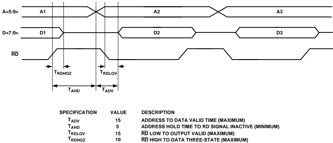
Figure 49. Parallel Port Read Timing Diagram
