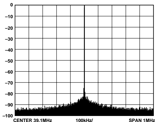
Figure 8. Narrowband SFDR, 39.1 MHz, 1 MHz BW, 300 MHz EXTCLK with REFCLK Multiply Bypassed
