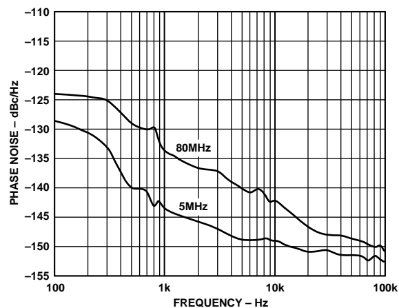
a. Residual Phase Noise 300 MHz Direct Clocking
