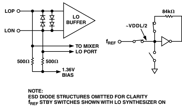
Figure 5. Equivalent Input of LO and REF Buffers
