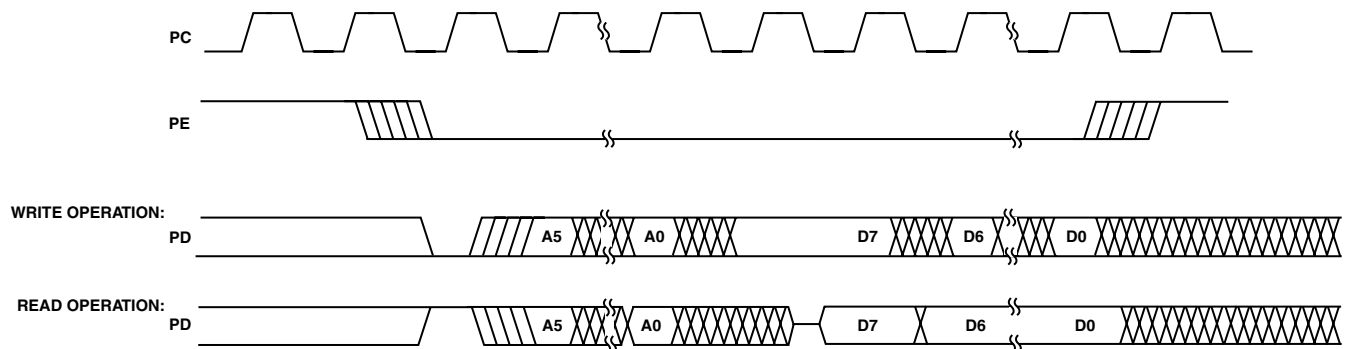
Figure 1. SPI Timing
