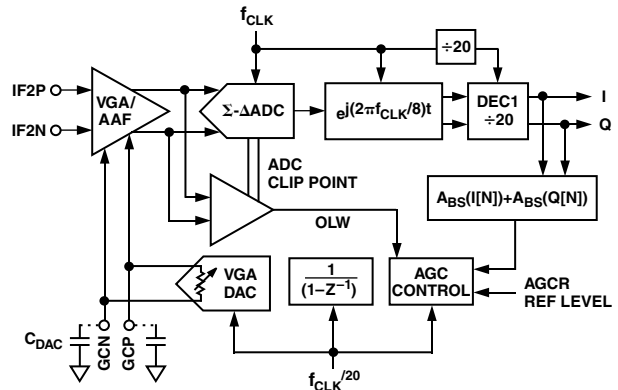
Figure 10. Functional Block Diagram of VGA and AGC
