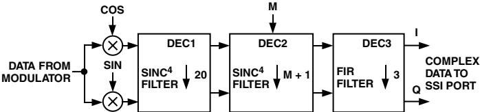
Figure 12. Decimation Filter Architecture
