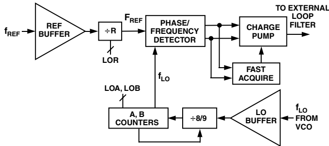
Figure 4. LO Synthesizer
