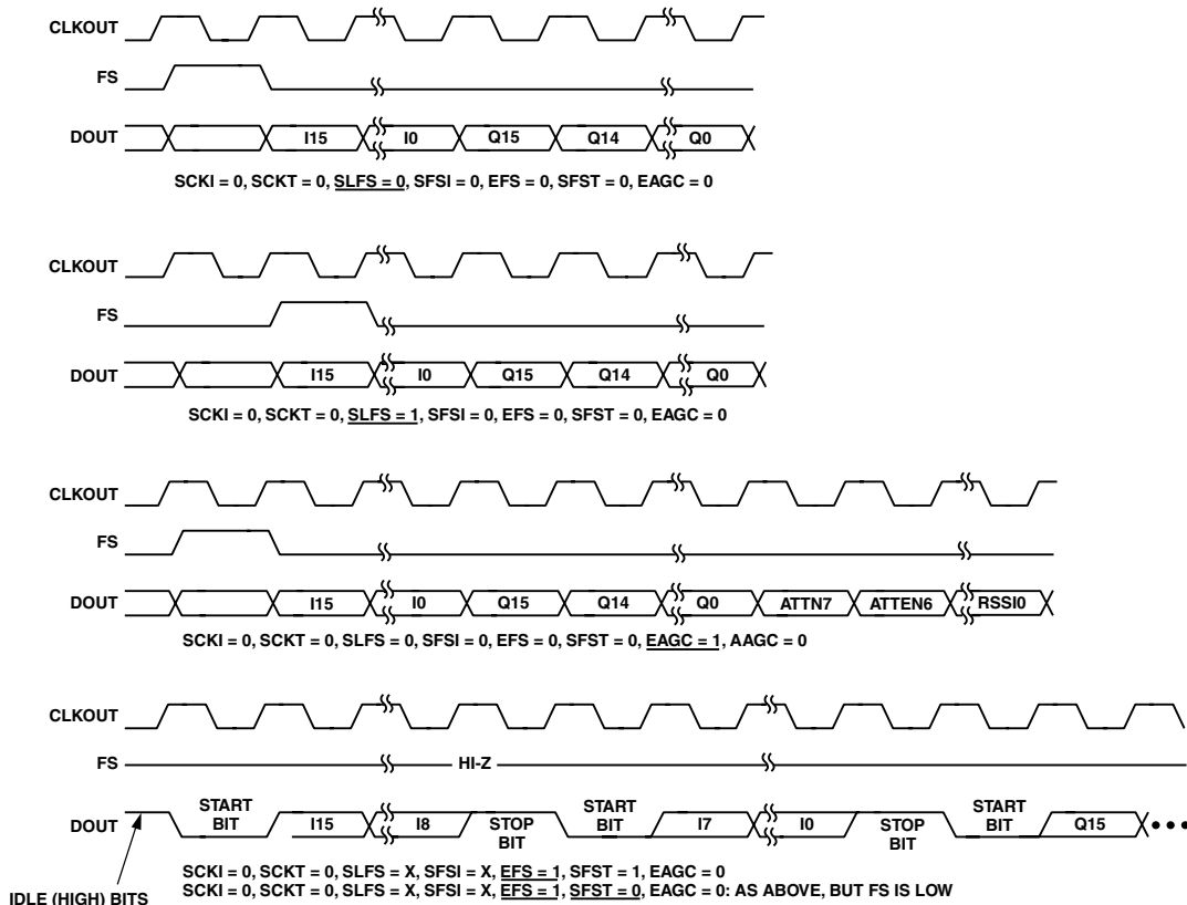
Figure 3a. SSI Timing for Several SSICR Settings with 16 Bit I/Q Data
