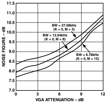
TPC 11a. Noise Figure vs. VGA Attenuation ( f_{CLK} = 13 MSPS)
