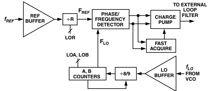
Figure 5. LO Synthesizer
