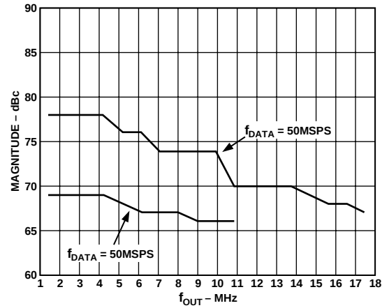
TPC 10. "Out of Band" SFDR vs. f_{OUT} @ f_{DATA} = 32 \text{ MSPS} and 50 MSPS
