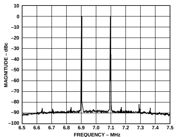
TPC 11. Dual Tone Spectral Plot @ f_{DATA} = 32 \text{ MSPS} , f_{OUT} = 6.9 \text{ MHz} and 7.1 MHz, 4x LPF
