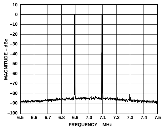
TPC 12. Dual Tone Spectral Plot @ f_{DATA} = 50 \text{ MSPS} , f_{OUT} = 6.9 \text{ MHz} and 7.1 MHz, 2x LPF
