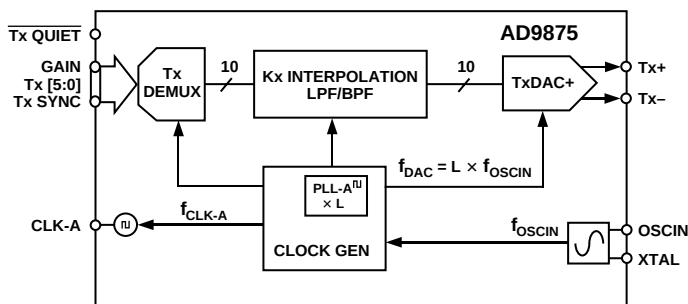
Figure 1. Transmit Path Block Diagram
