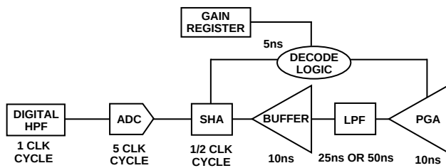
Figure 4. AGC Timing
