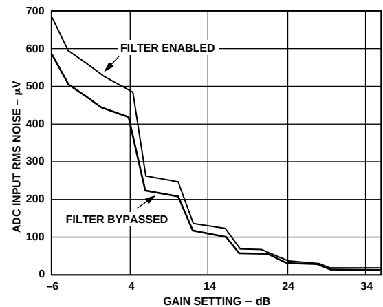
TPC 31. Rx Input Referred Noise vs. Gain @ f_{\text{ADC}} = 32 \text{ MSPS} , f_{\text{IN}} = 1 \text{ MHz}
