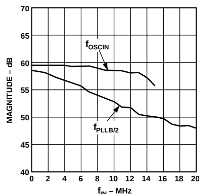
TPX 37. Rx Path SNR vs. f_{IN}
