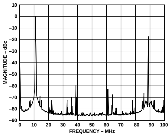
TPC 8. Single Tone Spectral Plot @ f_{DATA} = 50 \text{ MSPS} , f_{OUT} = 11 \text{ MHz} , 2x LPF
