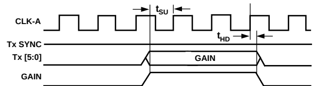
Figure 6. GAIN Programming
