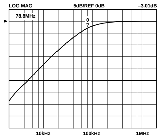
TPC 28. Rx HPF Frequency Response, f_{\text{ADC}} = 32 \text{ MHz}
