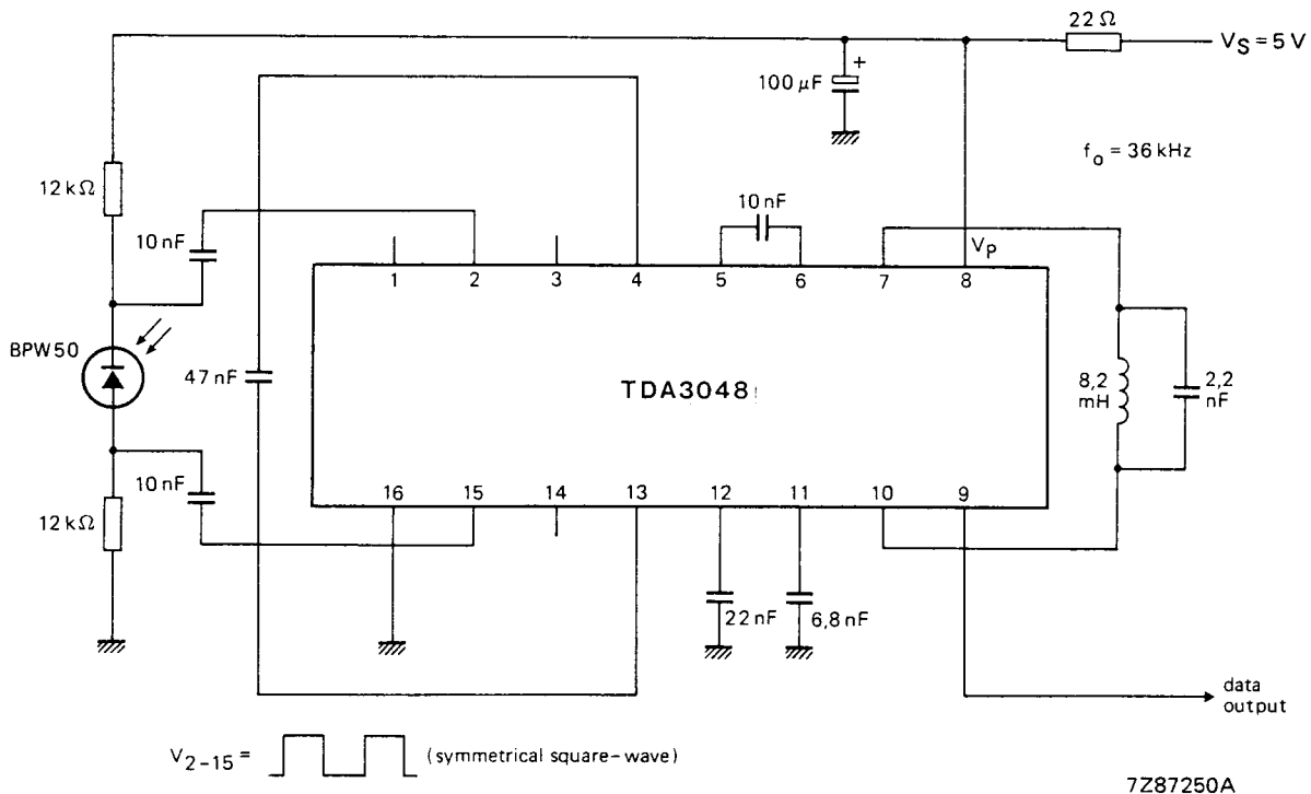
Fig. 4 Wide-band receiver with TDA3048.
