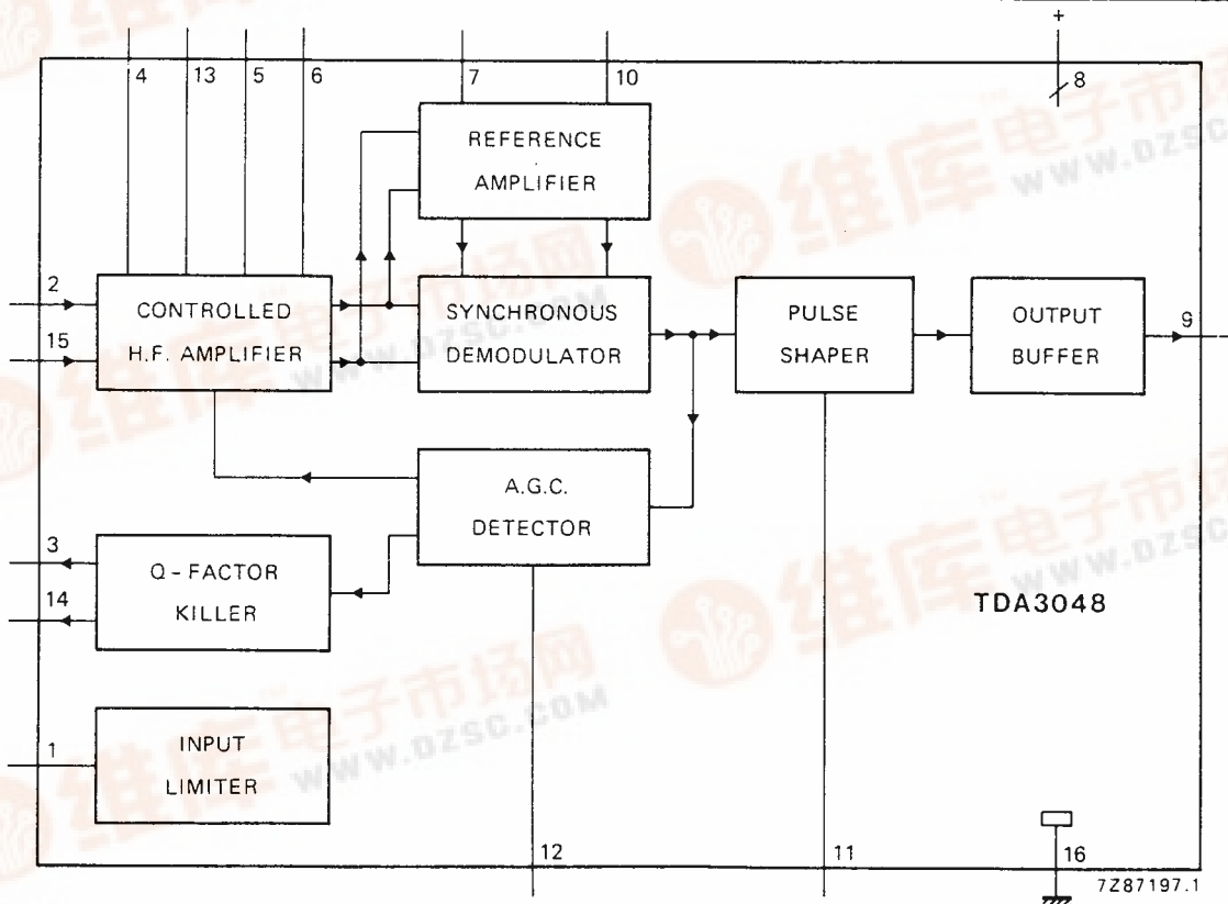
Fig. 1 Block diagram of TDA3048.
