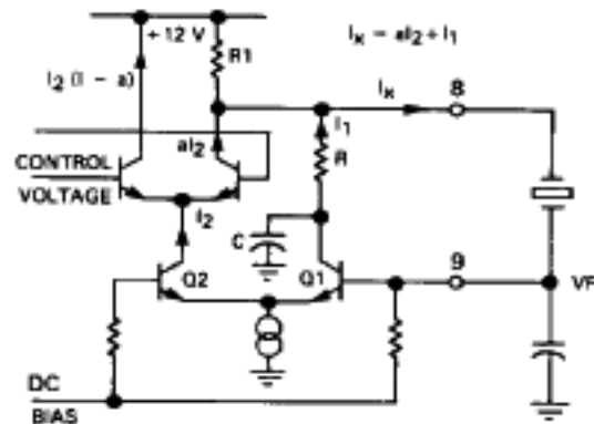
FIGURE 7 — VOLTAGE CONTROLLED OSCILLATOR (VCO)
