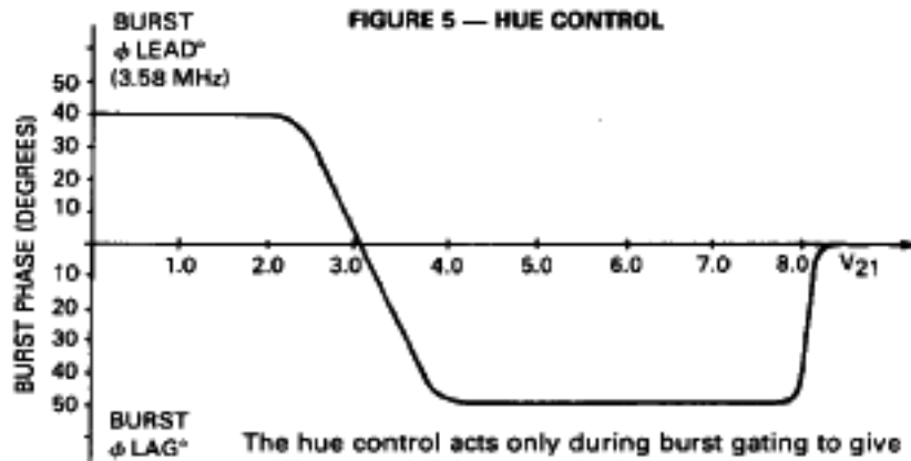
FIGURE 5 — HUE CONTROL
