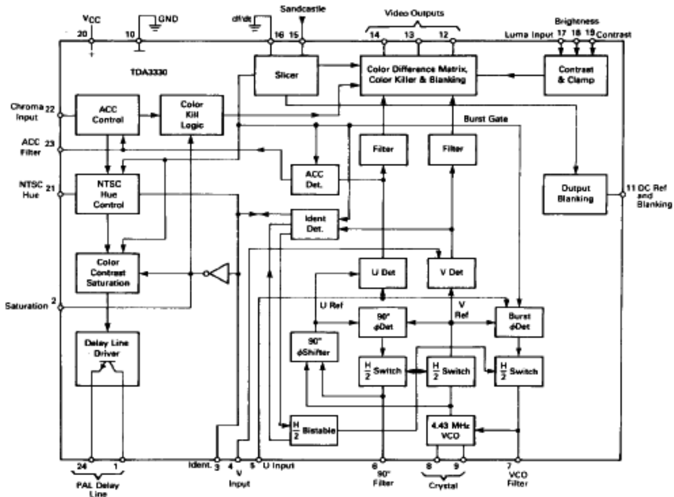
FIGURE 6 — BLOCK DIAGRAM
