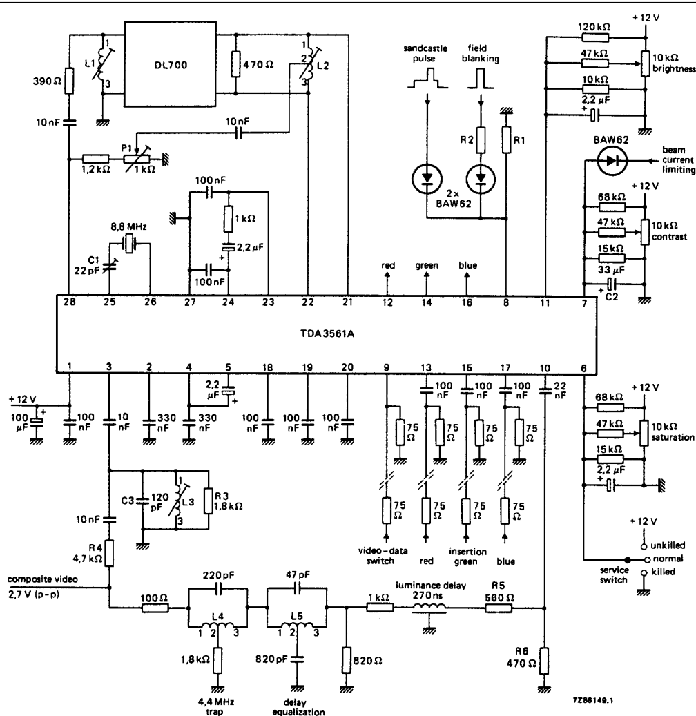
Fig.6 Application circuit.
