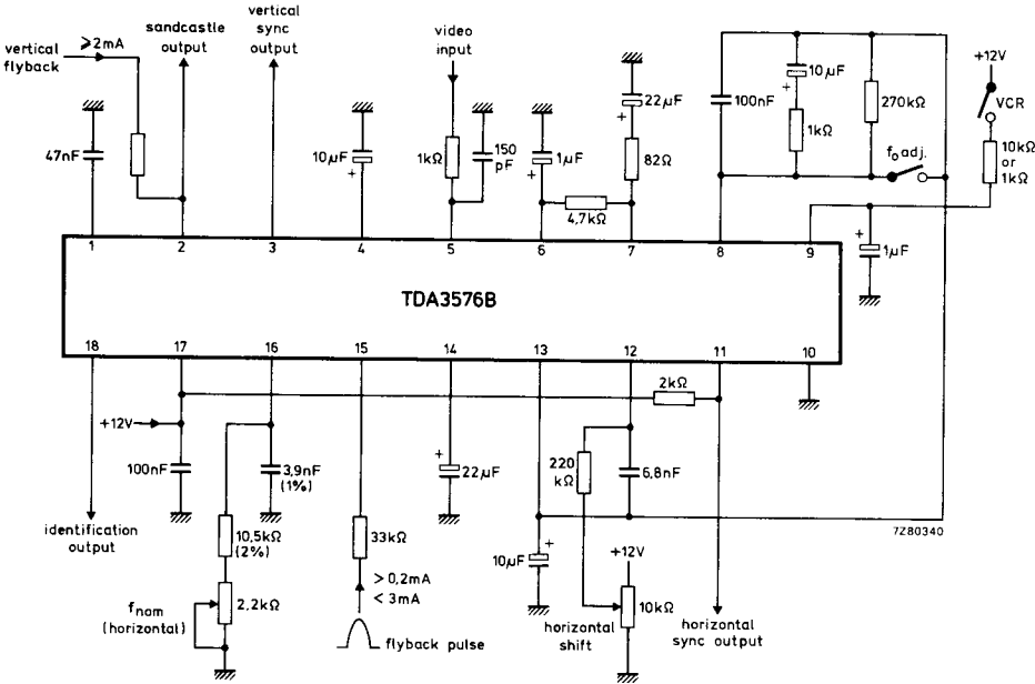
Fig. 3 Application circuit diagram.
