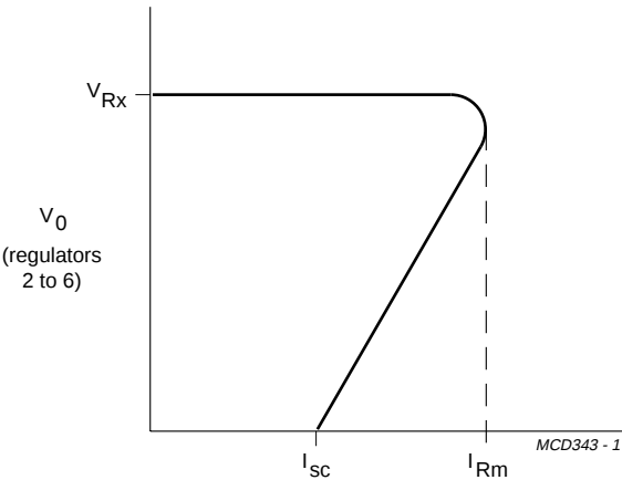
Fig.4 Foldback current protection behaviour.
