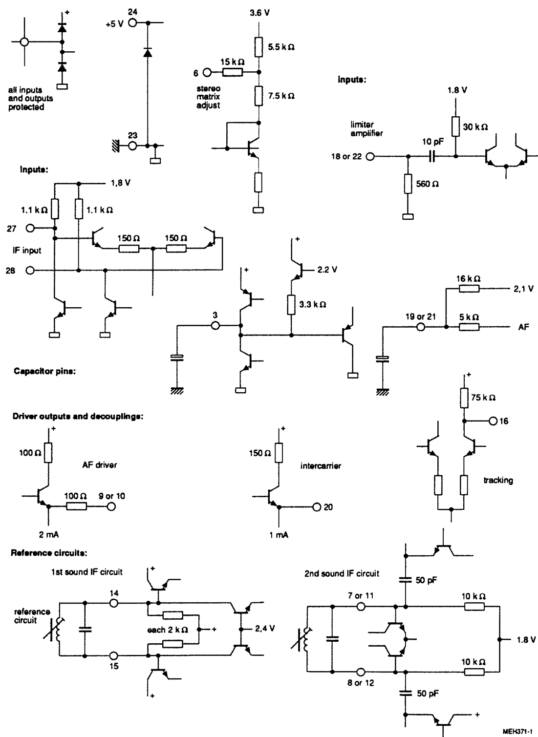
Fig.5 Internal circuits.
