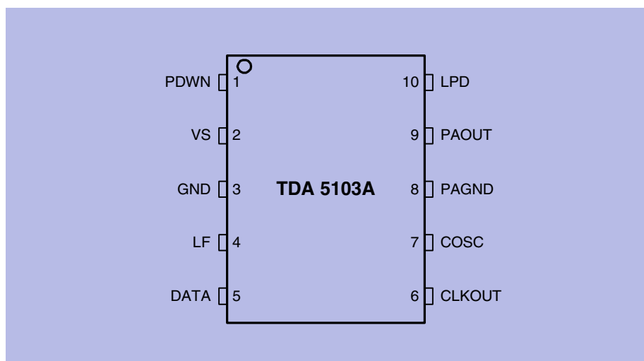
Figure 3-1 IC Pin Configuration
