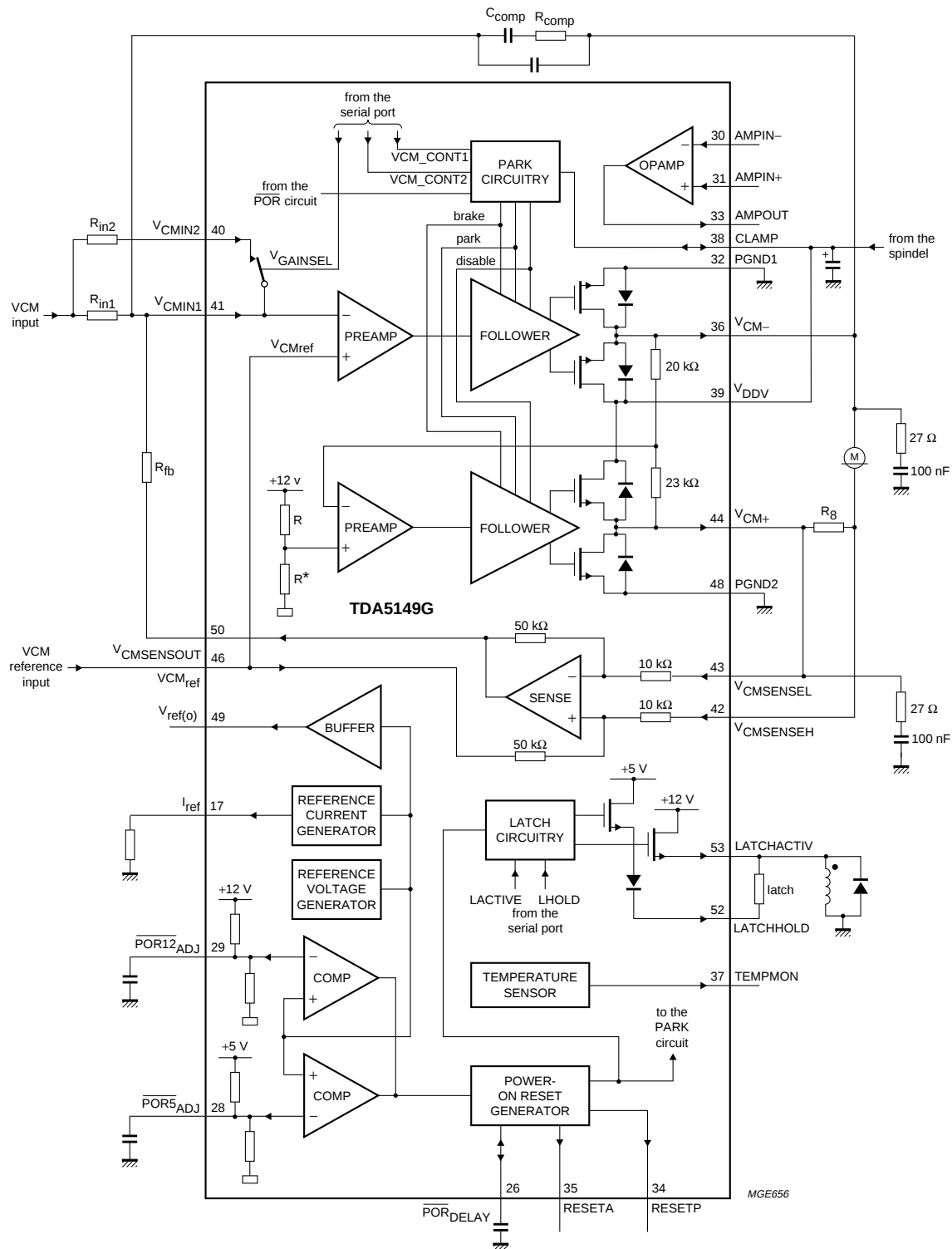
Fig.2 Block diagram of the VCM and RESET circuits.
