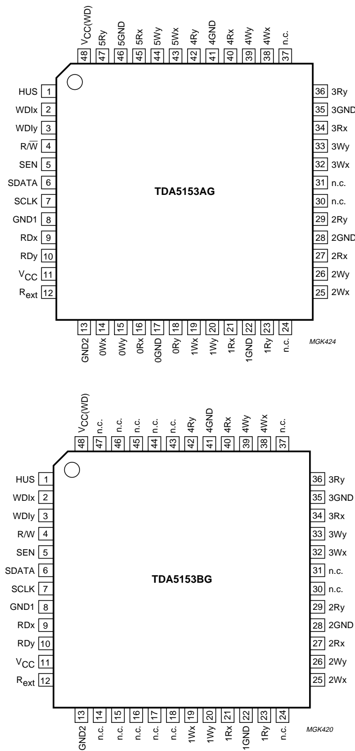
Fig.2 Pin configurations.
