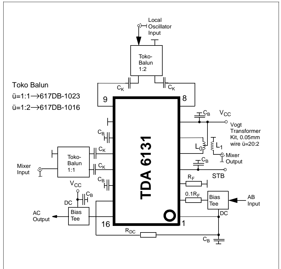
Figure 4-1 Test Circuit 1
