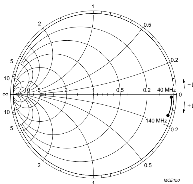
Fig.4 Input admittance ( S_{11} ) of the low band mixer (40 to 140 MHz); Y_0 = 20 mS.
