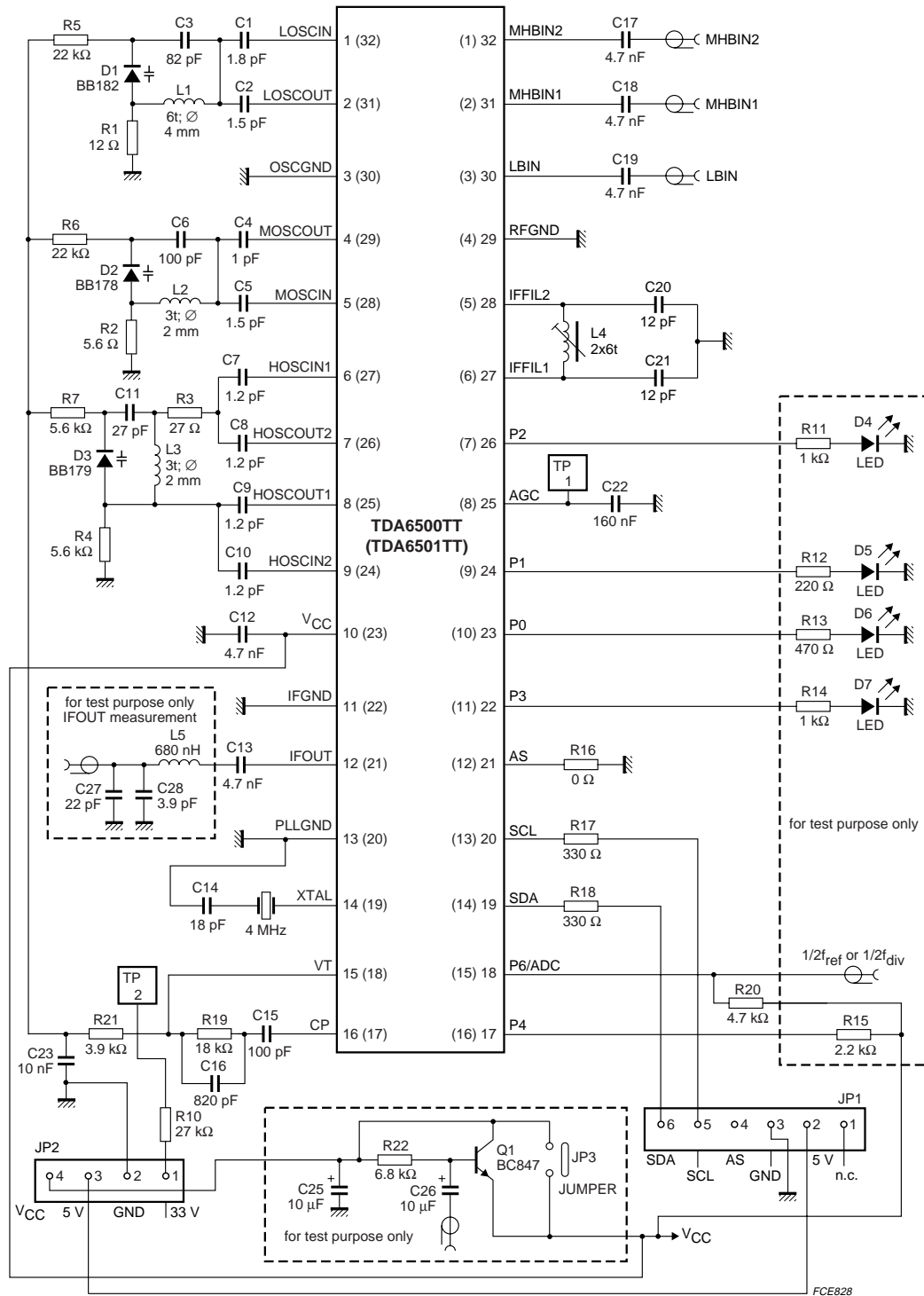
Fig.16 Measurement circuit for PAL on test jig.
