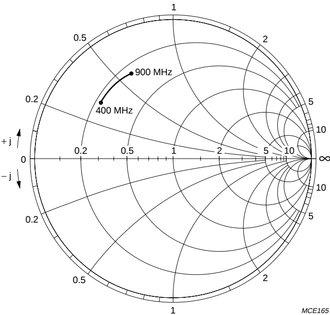
Fig.7 Input impedance ( S_{11} ) of the high band mixer (400 to 900 MHz); Z_0 = 100 \Omega .
