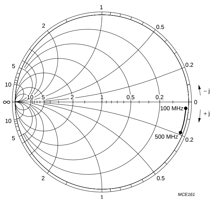
Fig.6 Input admittance ( S_{11} ) of the mid band mixer (100 to 500 MHz); Y_0 = 20 mS.
