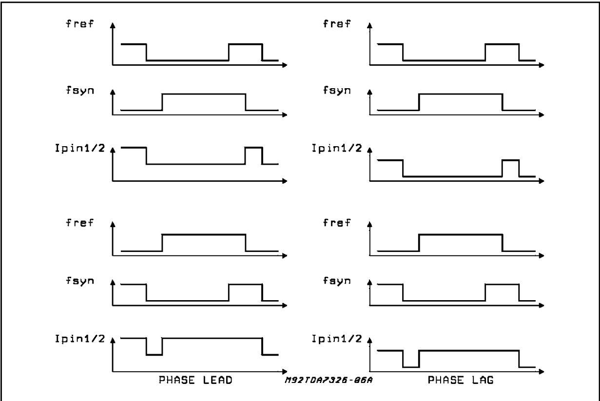
Figure 4: Phase comparator
