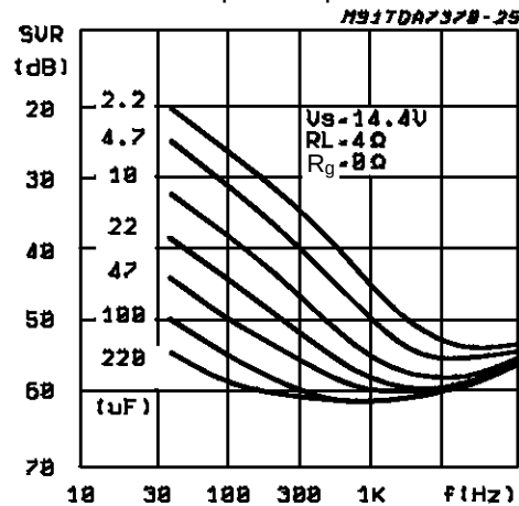
Figure 10: Supply Voltage Rejection vs. Frequency (Bridge) for different values of pin 6 capacitor.
