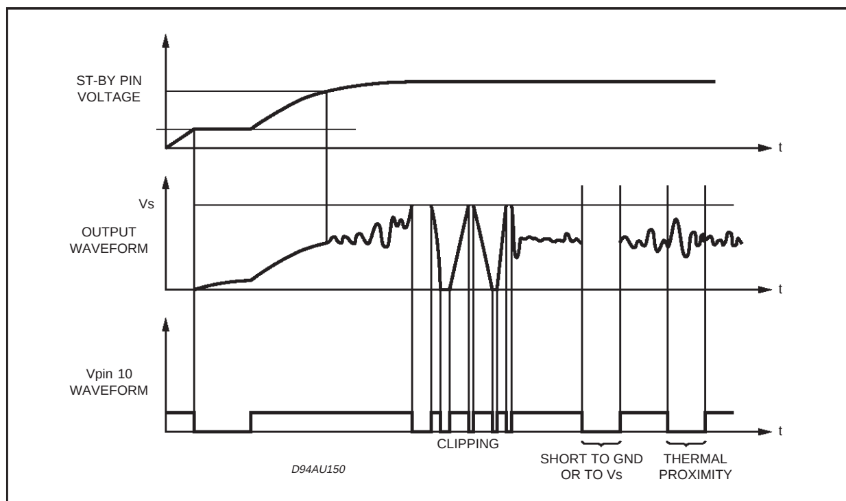
Figure 25: Waveforms
