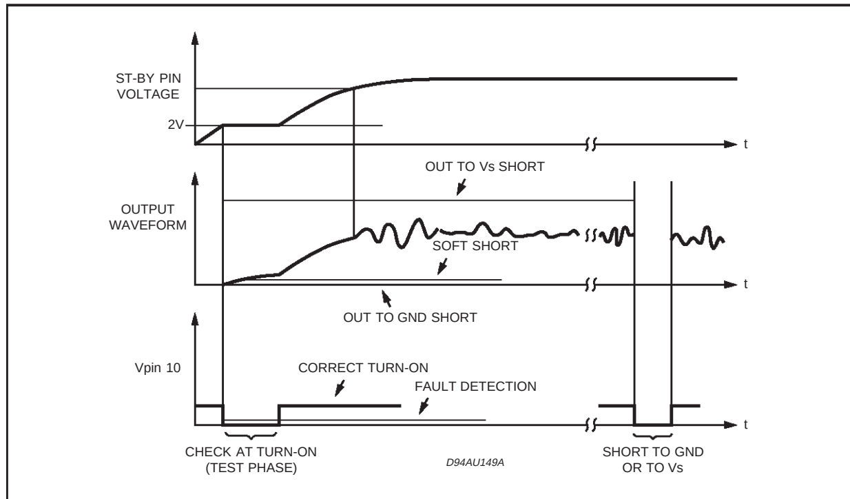
Figure 24: Fault Waveforms
