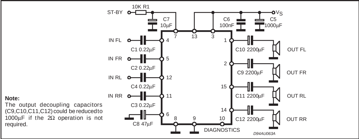
Figure 2: Double Bridge
