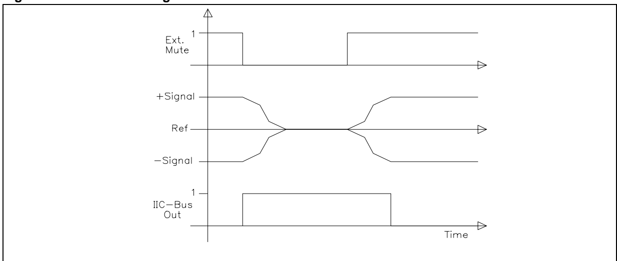
Figure 5. Soft Mute-Timing
