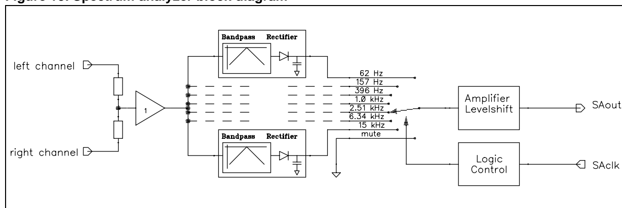
Figure 13. Spectrum analyzer block diagram
