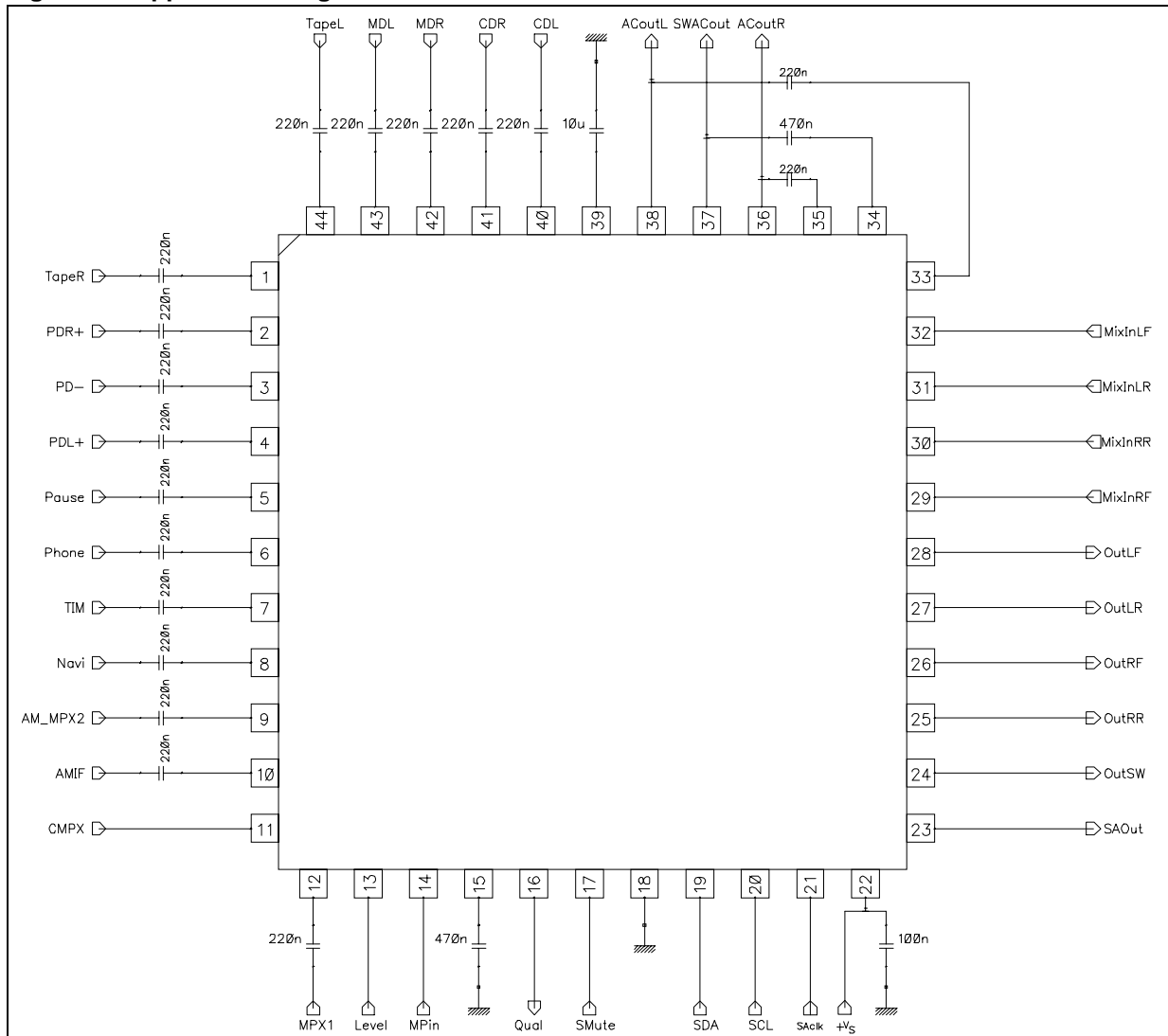
Figure 29. Application Diagram
