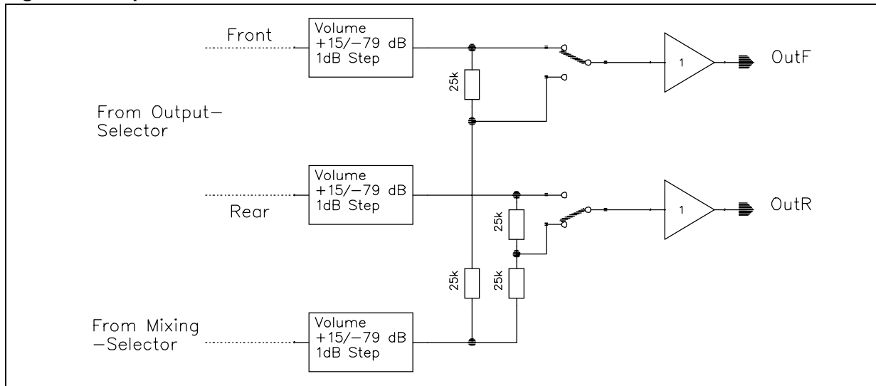
Figure 16. Output Selector
