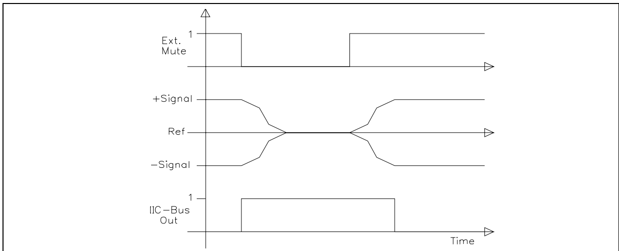
Figure 6. Softmute-Timing
