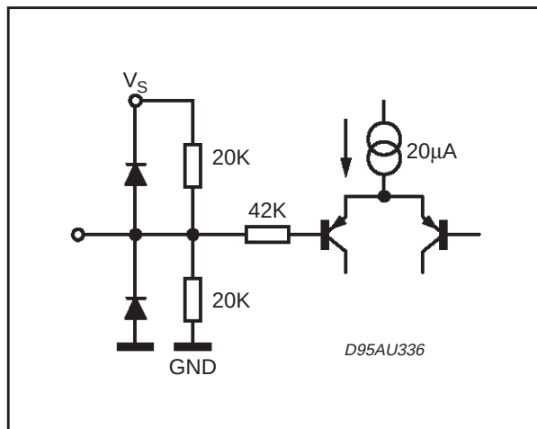
Figure 10. Pin: CREF
