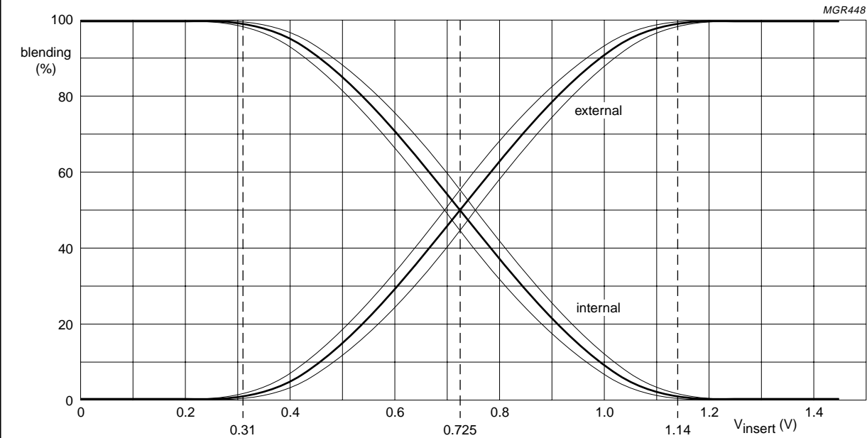
Fig.4 Blending characteristic (typical curve and minimum/maximum limits).
