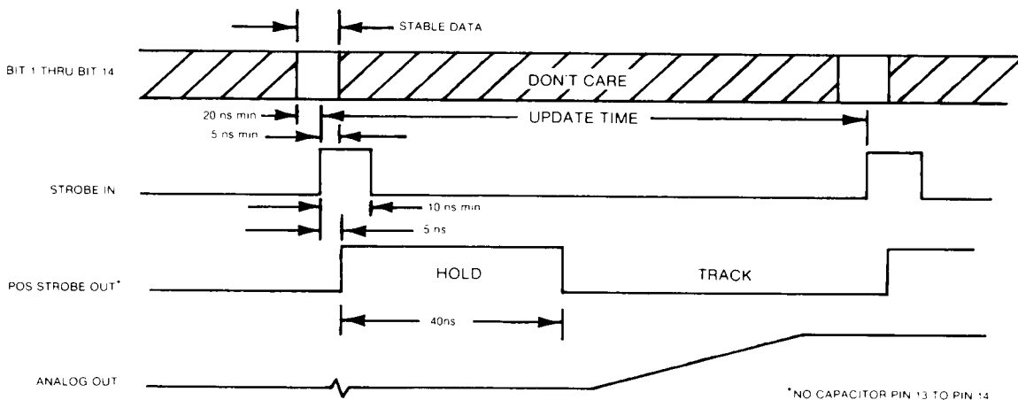
FIGURE 2. TIMING DIAGRAM
