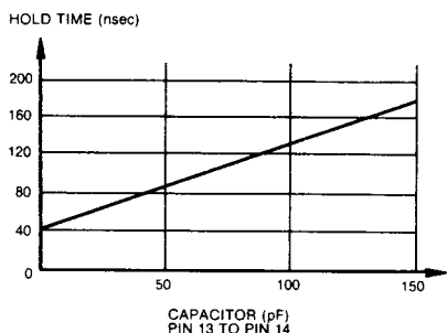
FIGURE 3. DELAY/HOLD TIME ADJUST
