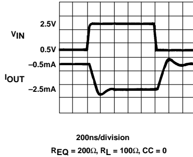
LSB Switching
