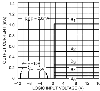
Bit Transfer Characteristics
