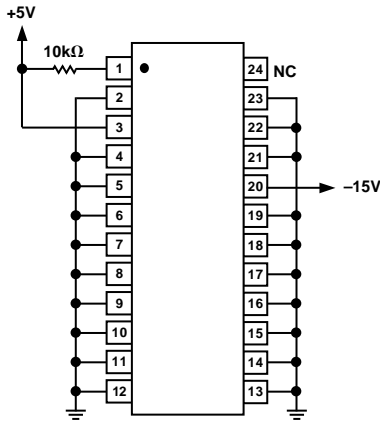
Figure 2. Burn-In Diagram
