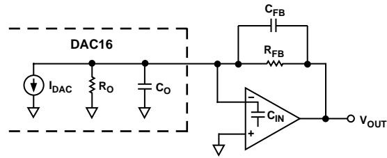
Figure 28. Compensating for the Feedback Pole
