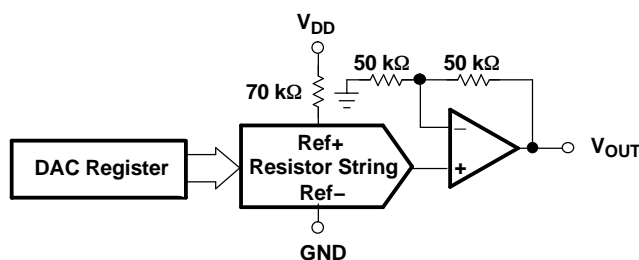
Figure 39. R-String DAC Architecture
