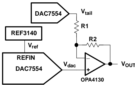
Figure 35. Low-cost, Wide-swing Voltage Generator for Control Loop Applications
