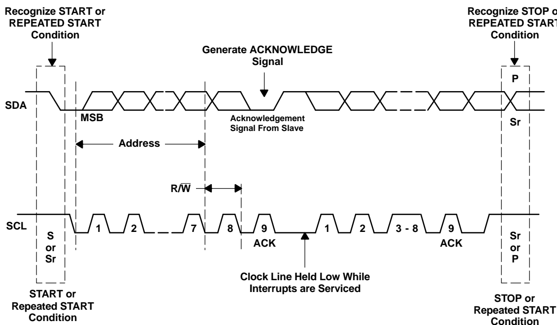
Figure 34. Bus Protocol
