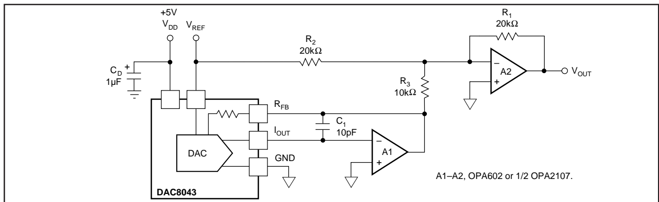
FIGURE 5. Bipolar Configuration.
