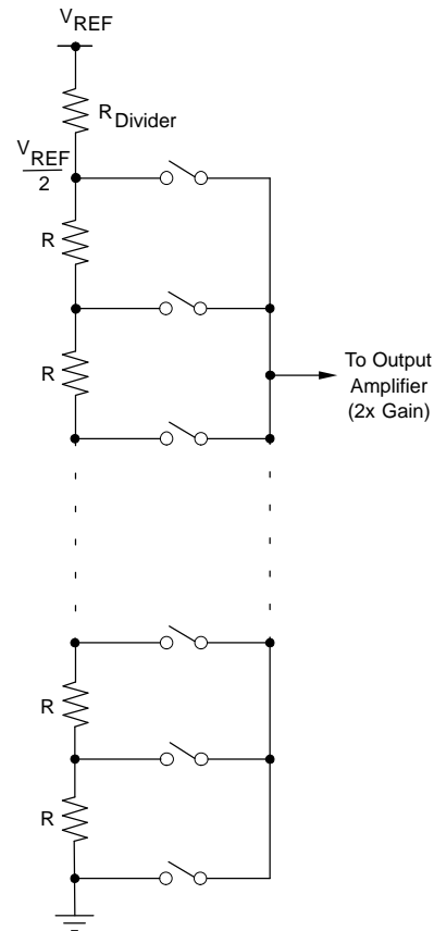
Figure 48. Resistor String
