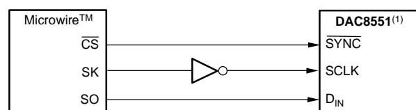
Figure 53. DAC8551 to Microwire Interface
