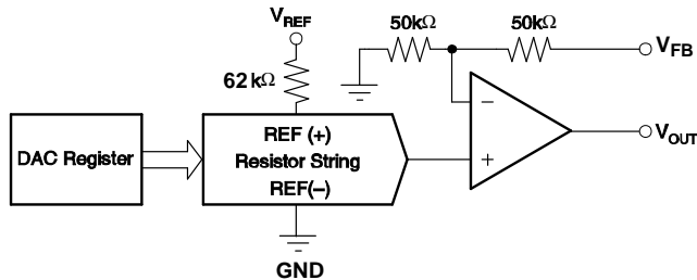
Figure 47. DAC8551 Architecture
